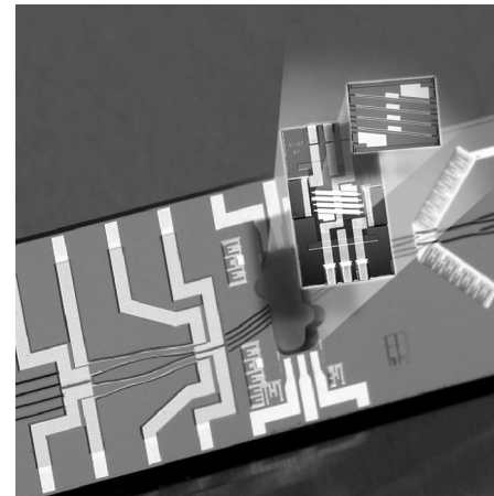
Figure 1. Hybrid integration concept of active (InP) and passive (silicon) components onto a silicon motherboard.
